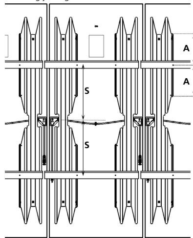
Fig. 2 Rear side: modules with „Hook-In“ mounting including joining elements
