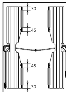
Fig. 6 Rear side of a shortened module with a length shorter than 1256 mm in „Hook-In” mounting variant
