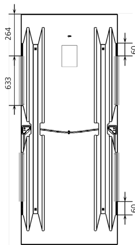
Fig. 5 Module rear side „In-Joint” variant
